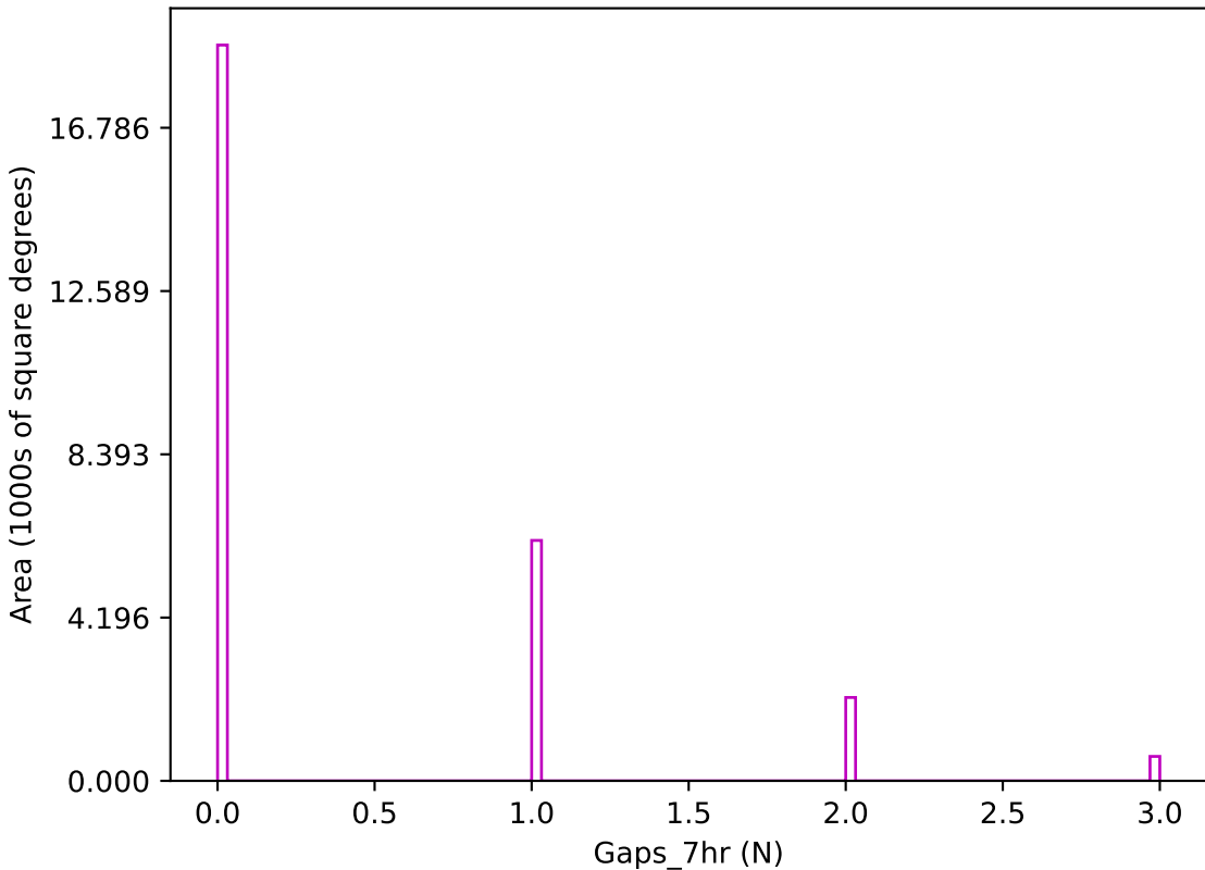
too_elab_r64_d3_ugrizy_v3.4_10yrs z band: Gaps_7hr
