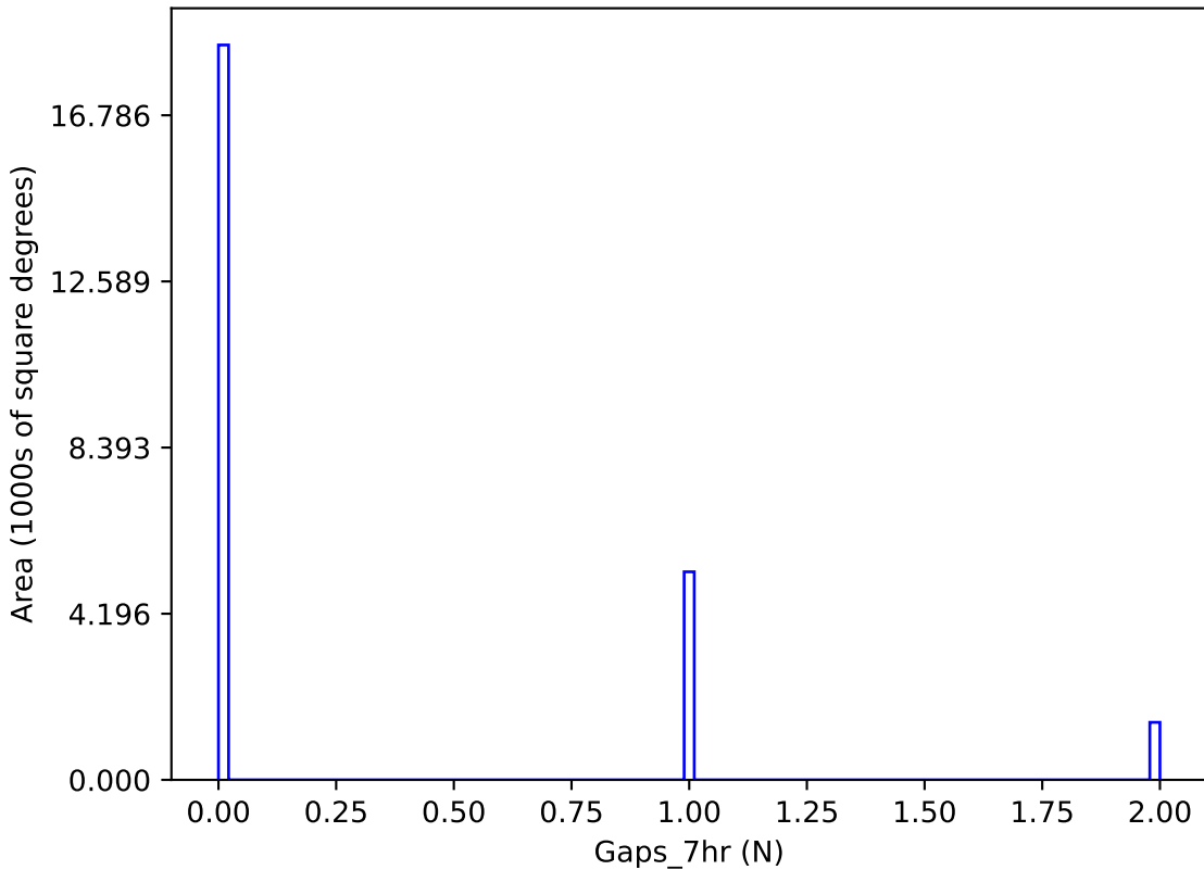
too_elab_r64_d3_ugrizy_v3.4_10yrs y band: Gaps_7hr
