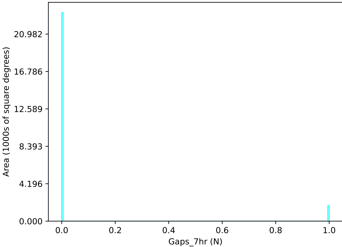
too_elab_r64_d3_ugrizy_v3.4_10yrs u band: Gaps_7hr
