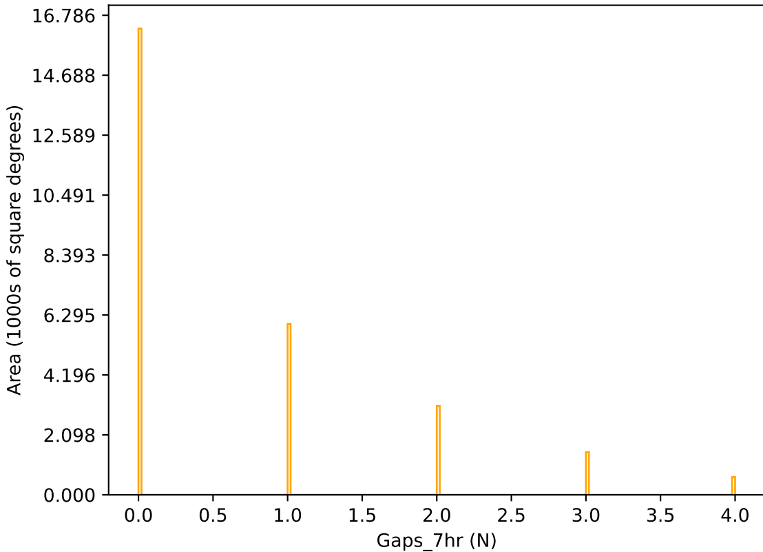
too_elab_r64_d3_ugrizy_v3.4_10yrs r band: Gaps_7hr
