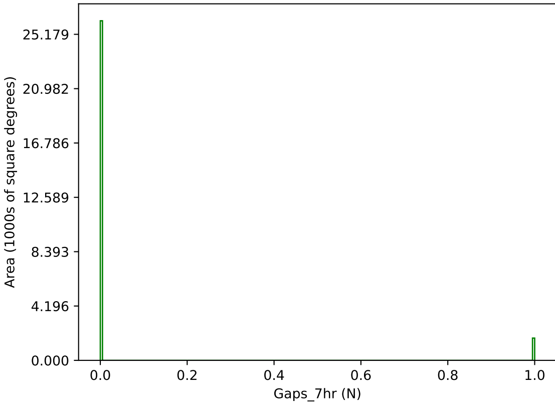
too_elab_r64_d3_ugrizy_v3.4_10yrs g band: Gaps_7hr
