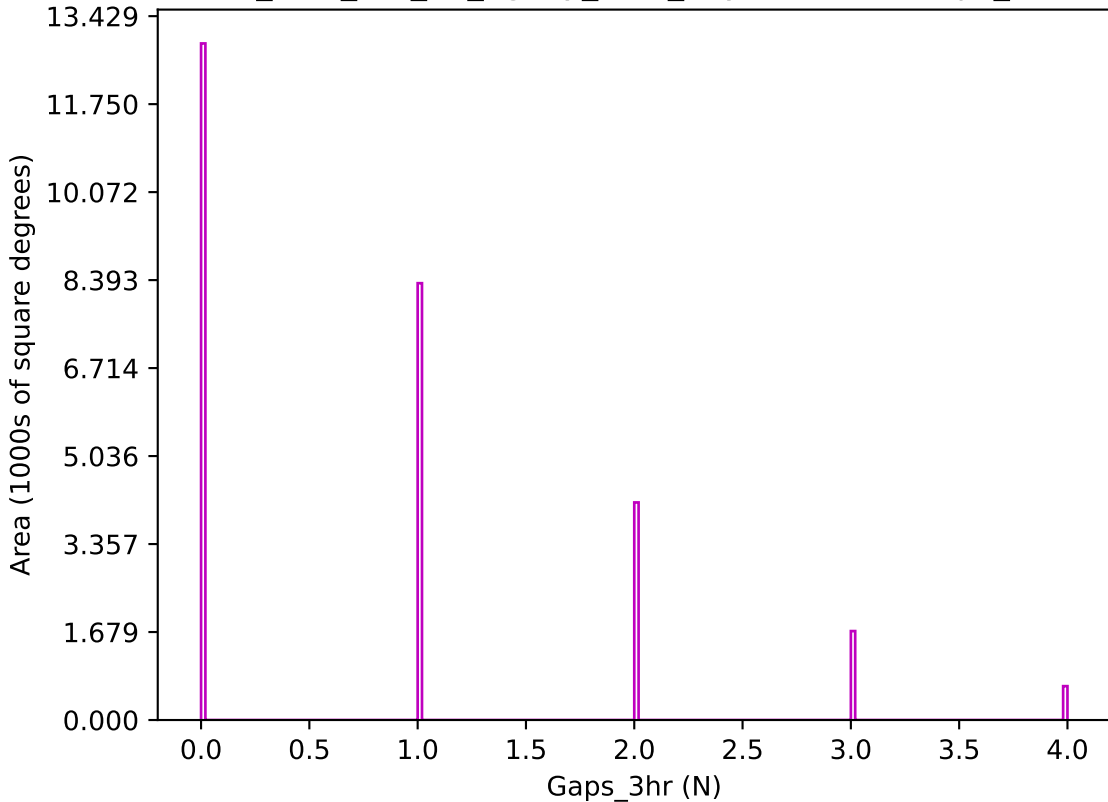
too_elab_r64_d3_ugrizy_v3.4_10yrs z band: Gaps_3hr
