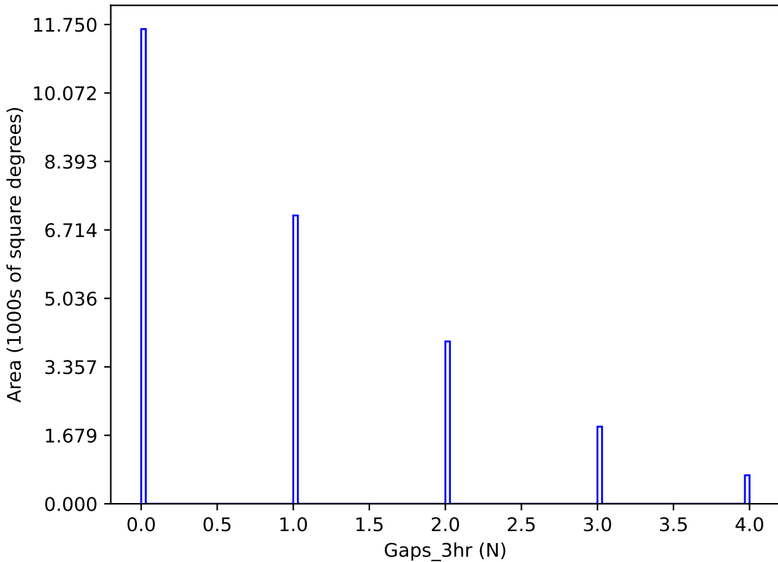
too_elab_r64_d3_ugrizy_v3.4_10yrs y band: Gaps_3hr
