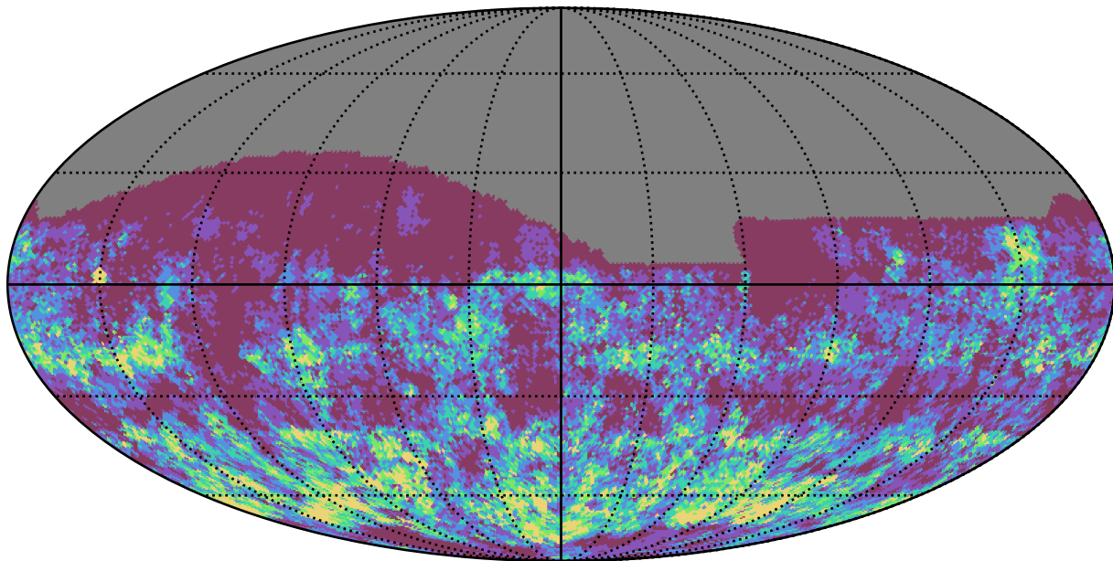
too_elab_r64_d3_ugrizy_v3.4_10yrs r band: Gaps_3hr
