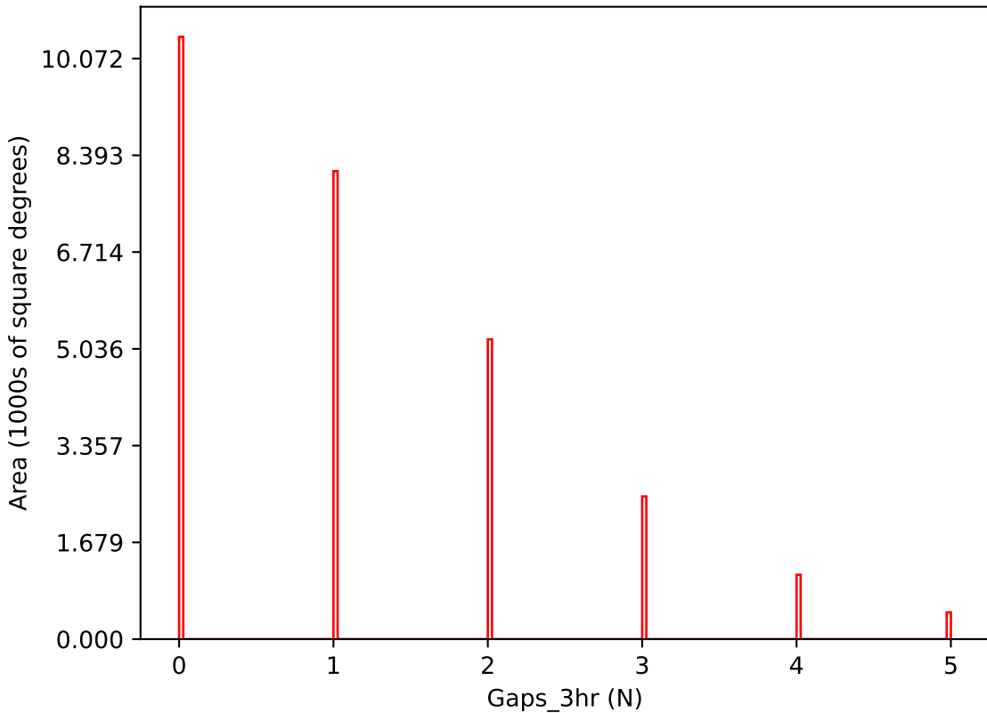
too_elab_r64_d3_ugrizy_v3.4_10yrs i band: Gaps_3hr
