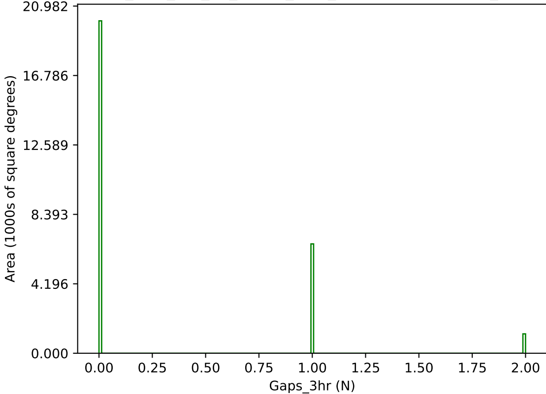
too_elab_r64_d3_ugrizy_v3.4_10yrs g band: Gaps_3hr
