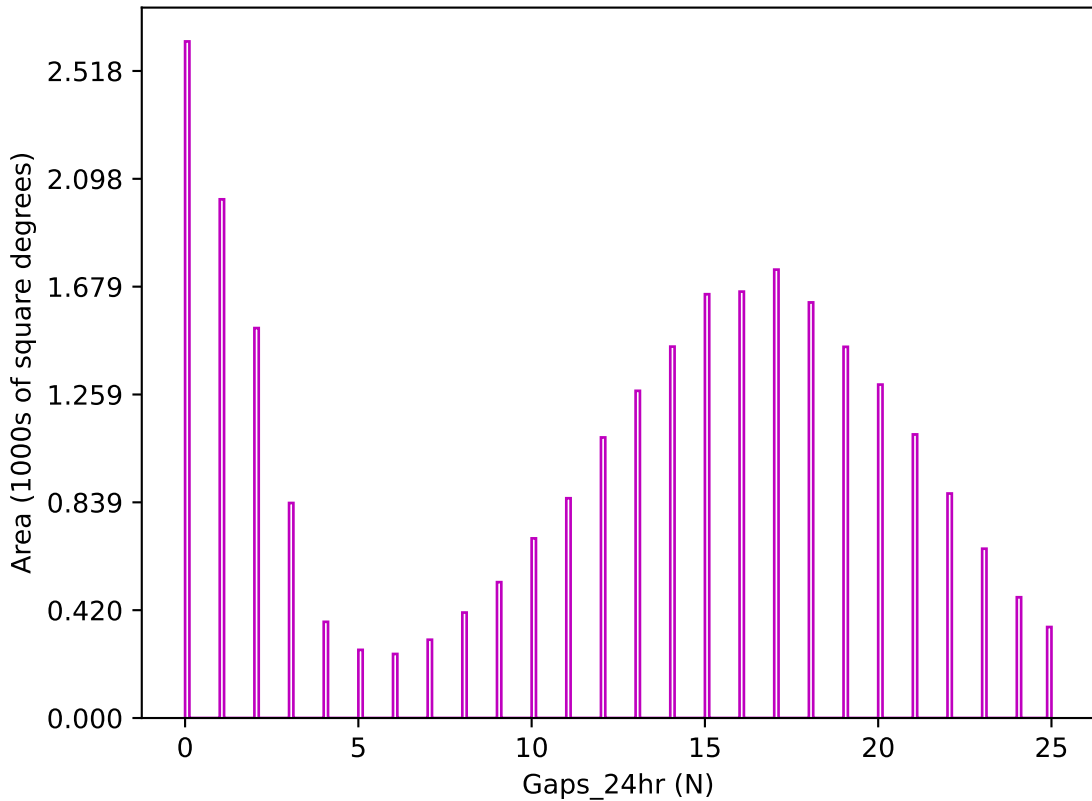
too_elab_r64_d3_ugrizy_v3.4_10yrs z band: Gaps_24hr
