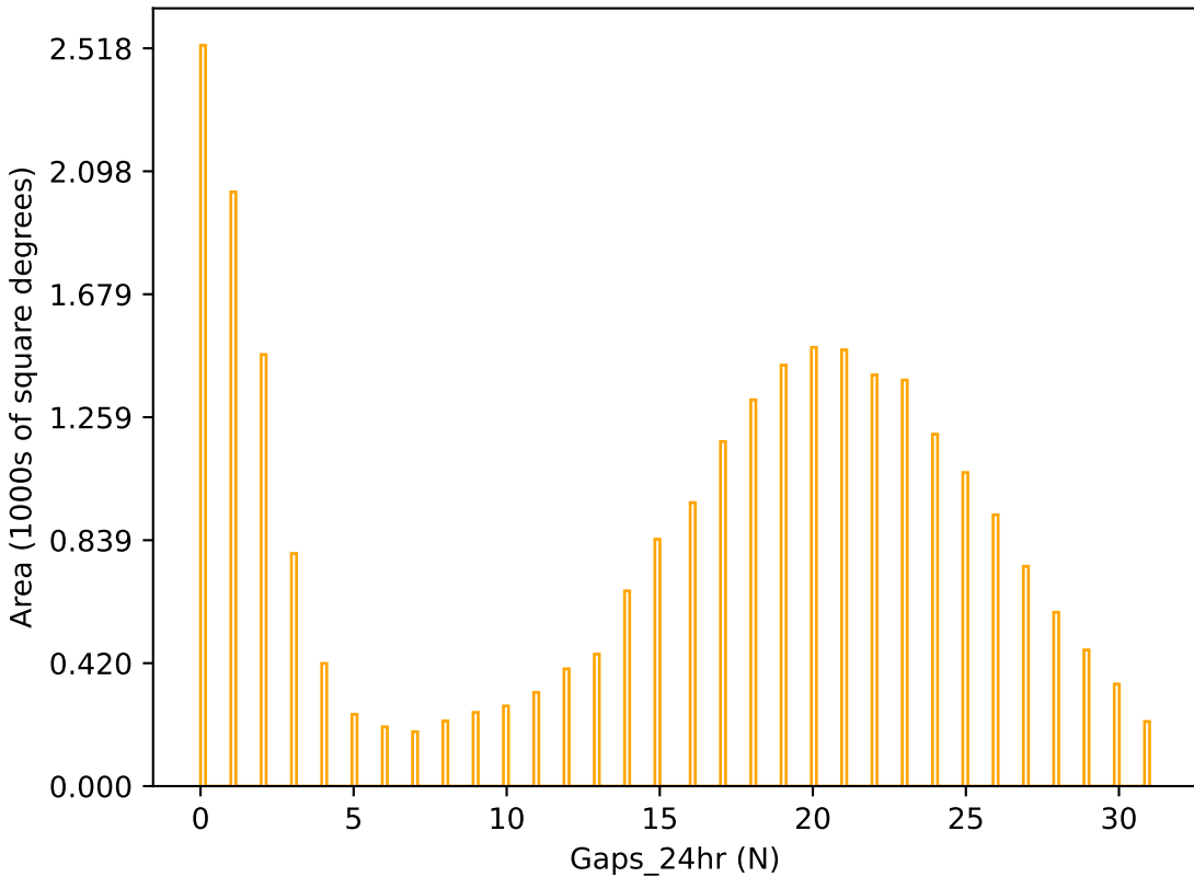
too_elab_r64_d3_ugrizy_v3.4_10yrs r band: Gaps_24hr
