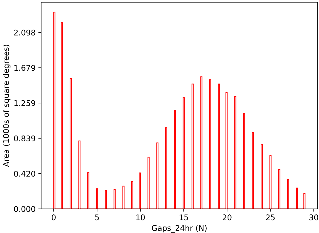
too_elab_r64_d3_ugrizy_v3.4_10yrs i band: Gaps_24hr
