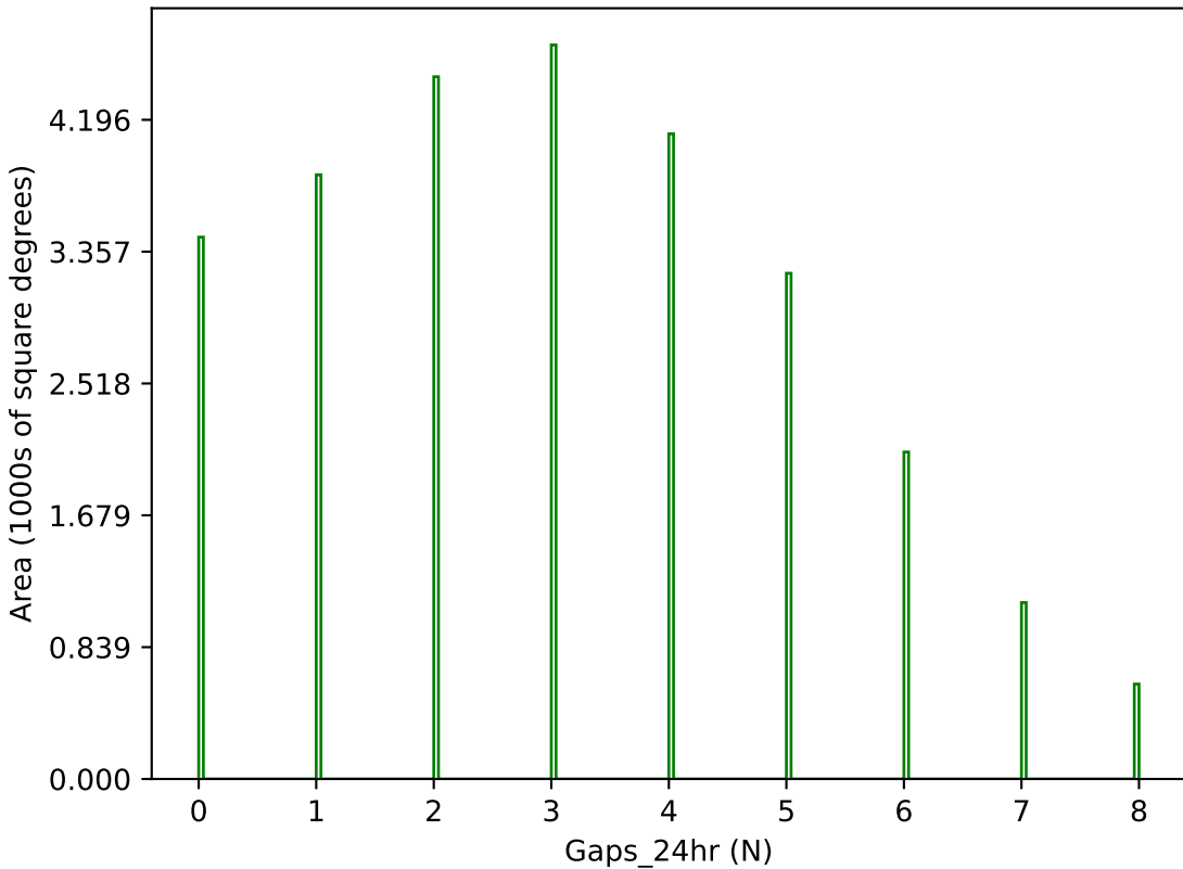
too_elab_r64_d3_ugrizy_v3.4_10yrs g band: Gaps_24hr
