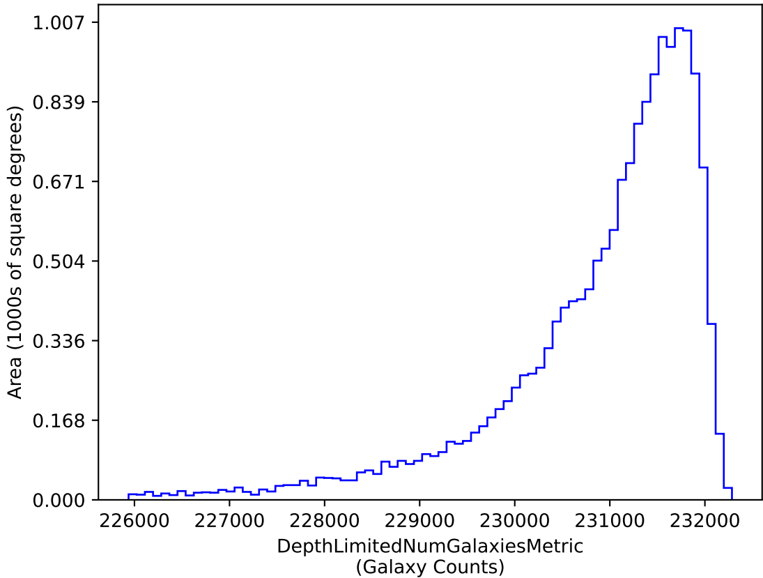
too_elab_r64_d3_ugrizy_v3.4_10yrs i band galaxies non-DD: DepthLimitedNumGalaxiesMetric
