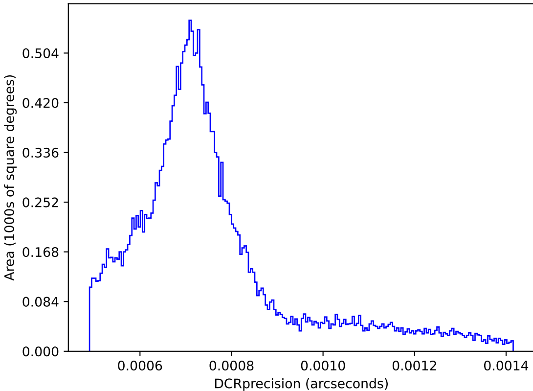
too_elab_r64_d3_ugrizy_v3.4_10yrs : DCRprecision
