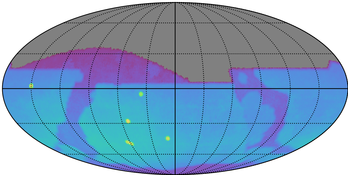
too_elab_r64_d3_ugrizy_v3.4_10yrs : Brown Dwarf, L7
