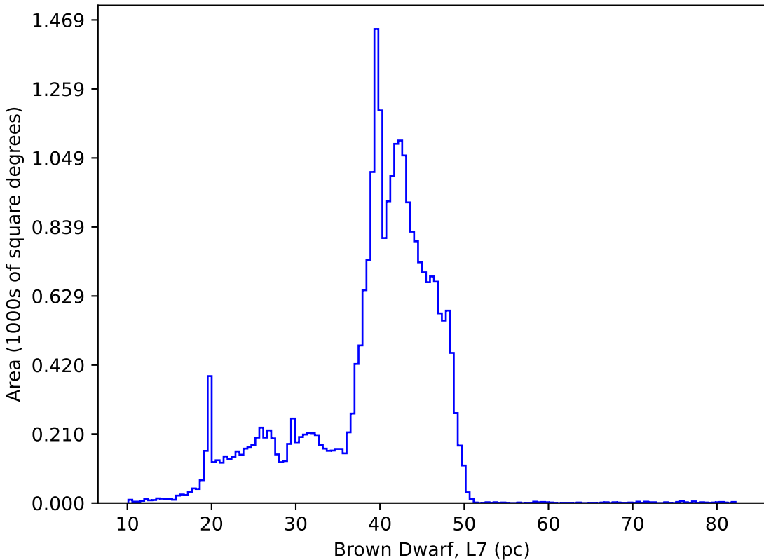
too_elab_r64_d3_ugrizy_v3.4_10yrs : Brown Dwarf, L7
