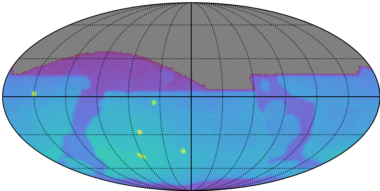
too_elab_r64_d3_ugrizy_v3.4_10yrs : Brown Dwarf, L4
