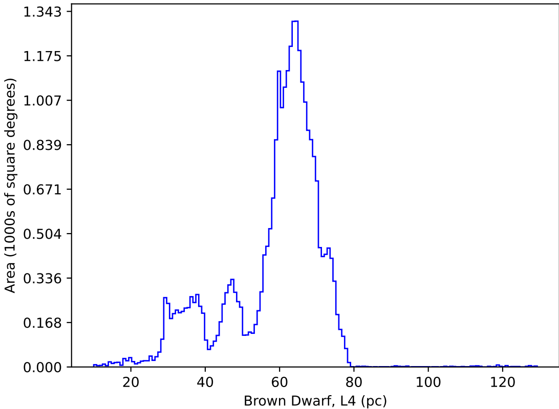
too_elab_r64_d3_ugrizy_v3.4_10yrs : Brown Dwarf, L4
