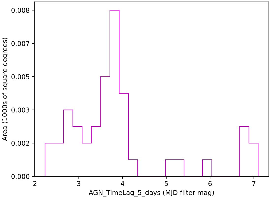
too_elab_r64_d3_ugrizy_v3.4_10yrs z band: AGN_TimeLag_5_days
