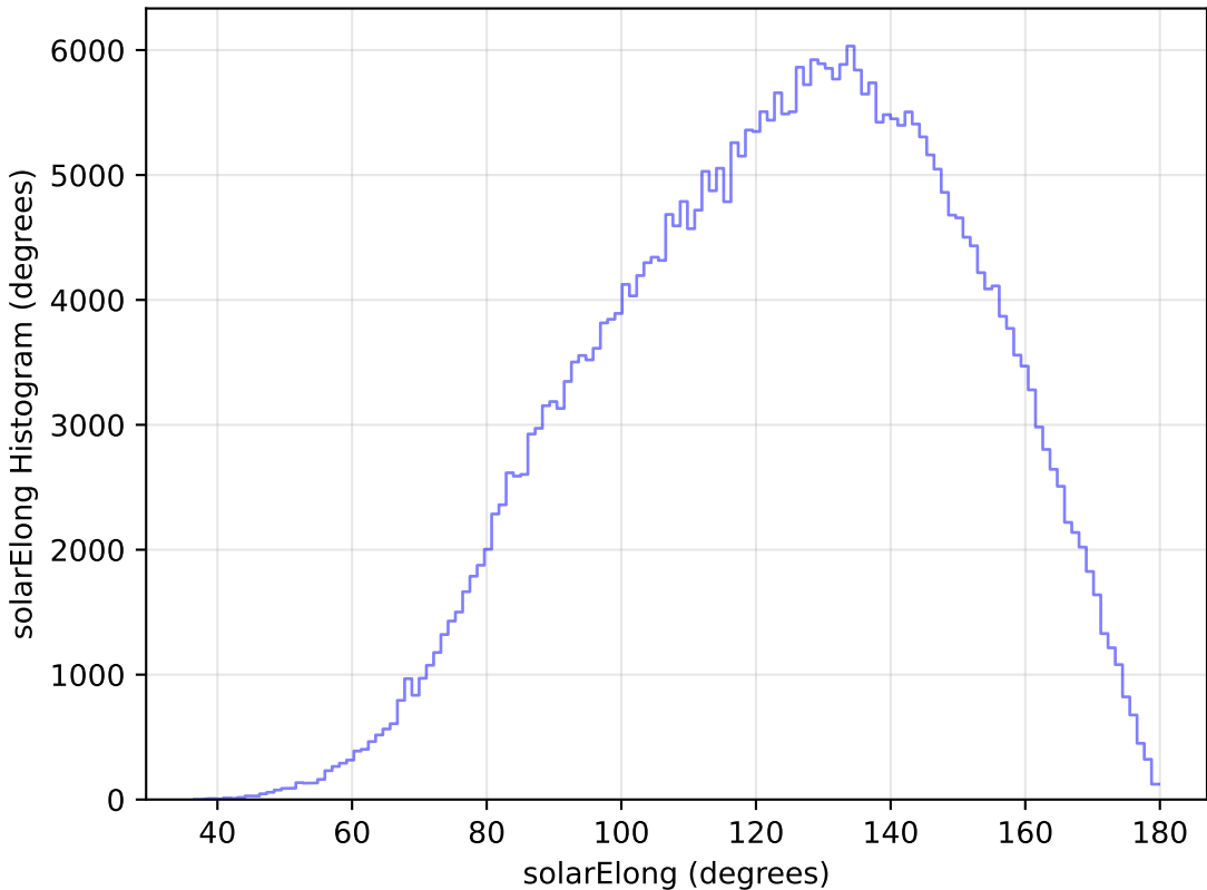
too_elab_r64_d3_ugrizy_v3.4_10yrs WFD y band: solarElong Histogram
