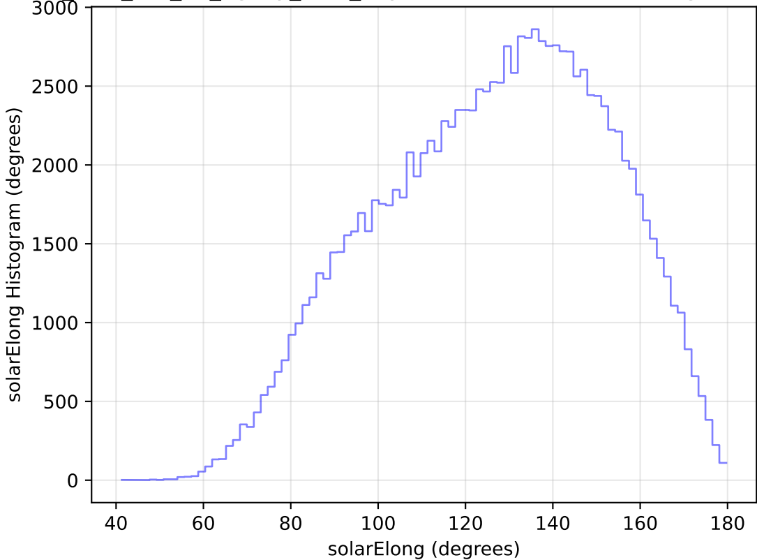
too_elab_r64_d3_ugrizy_v3.4_10yrs WFD u band: solarElong Histogram
