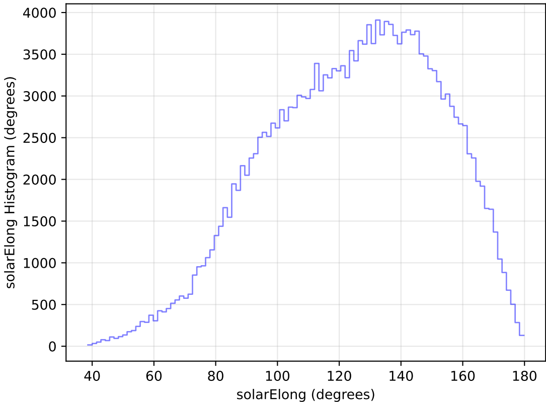
too_elab_r64_d3_ugrizy_v3.4_10yrs WFD g band: solarElong Histogram
