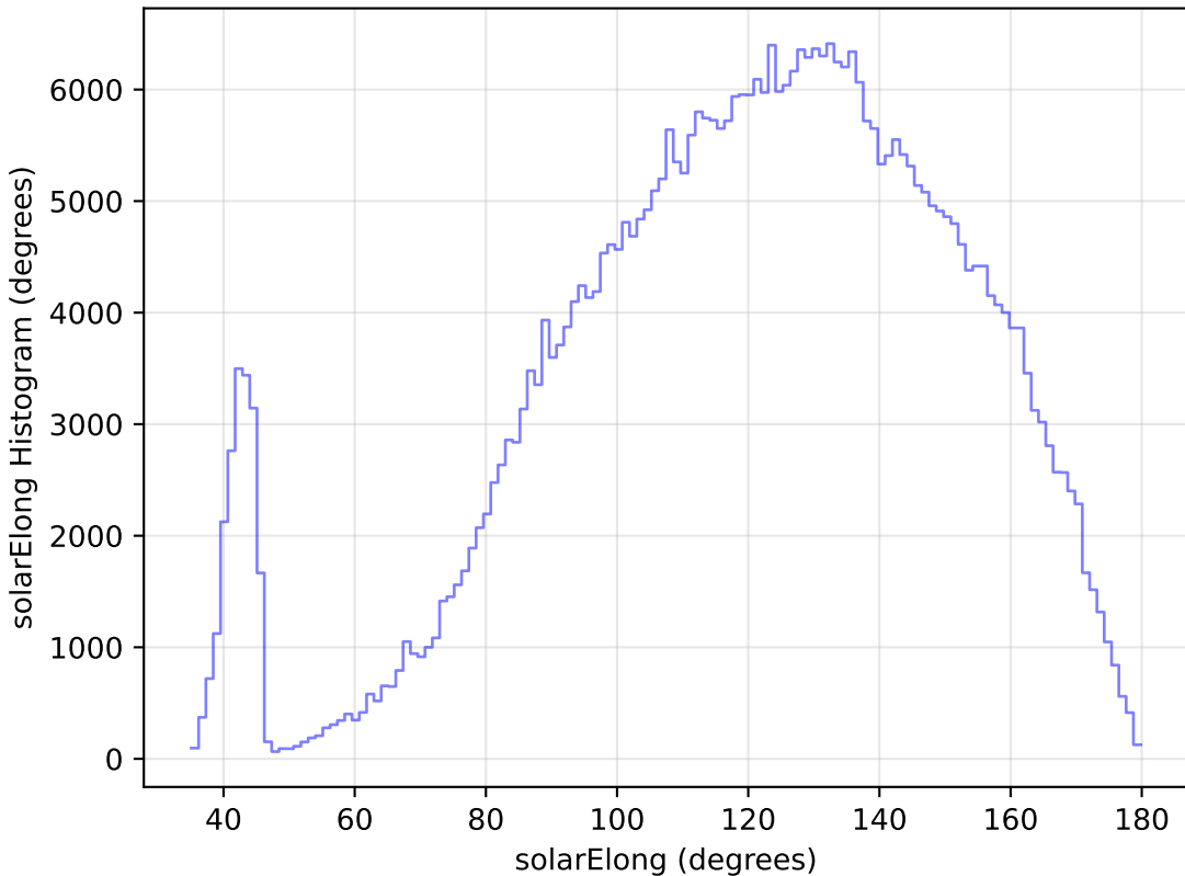
too_elab_r64_d3_ugrizy_v3.4_10yrs All sky z band: solarElong Histogram
