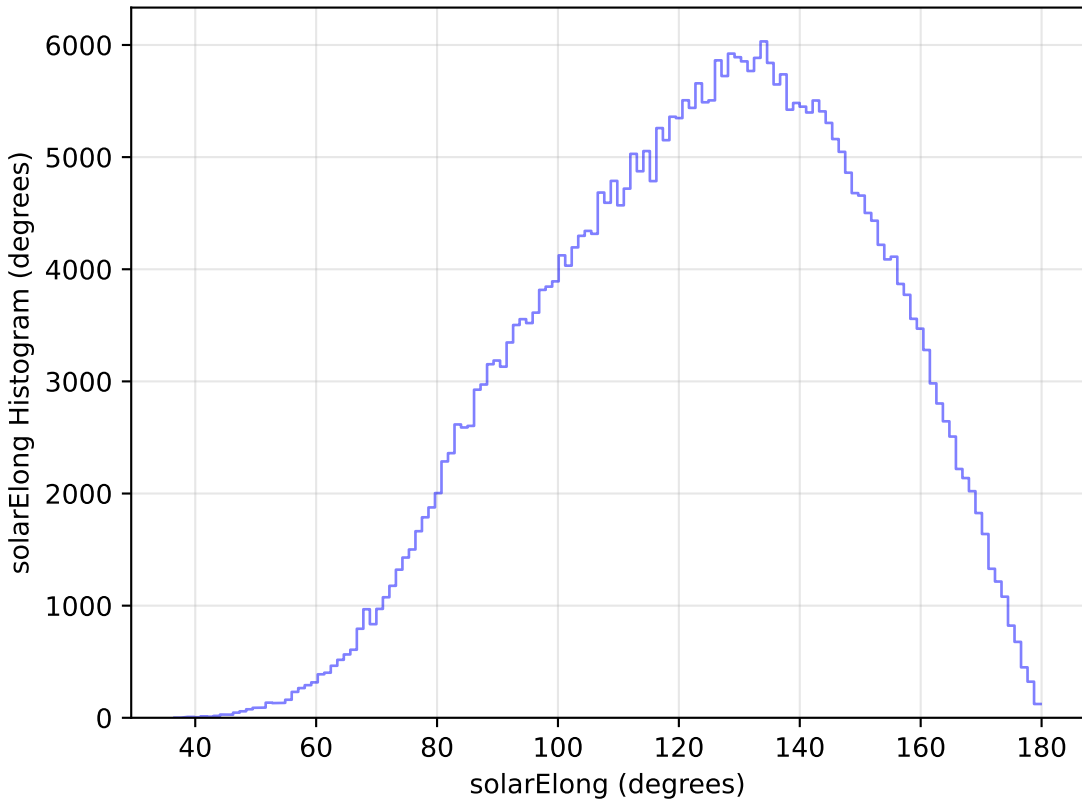
too_elab_r64_d3_ugrizy_v3.4_10yrs All sky y band: solarElong Histogram
