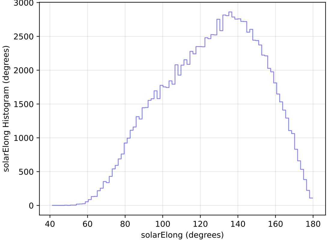
too_elab_r64_d3_ugrizy_v3.4_10yrs All sky u band: solarElong Histogram
