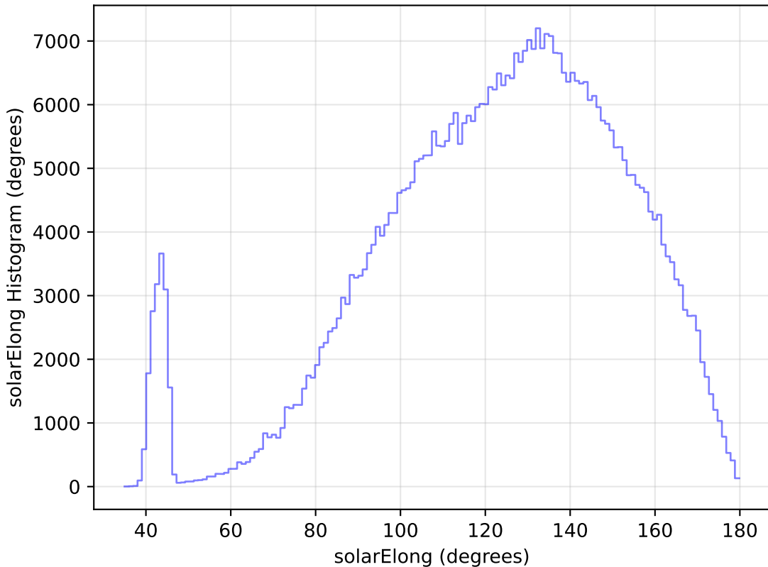
too_elab_r64_d3_ugrizy_v3.4_10yrs All sky r band: solarElong Histogram
