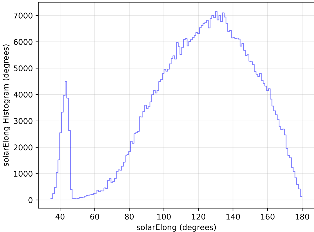
too_elab_r64_d3_ugrizy_v3.4_10yrs All sky i band: solarElong Histogram
