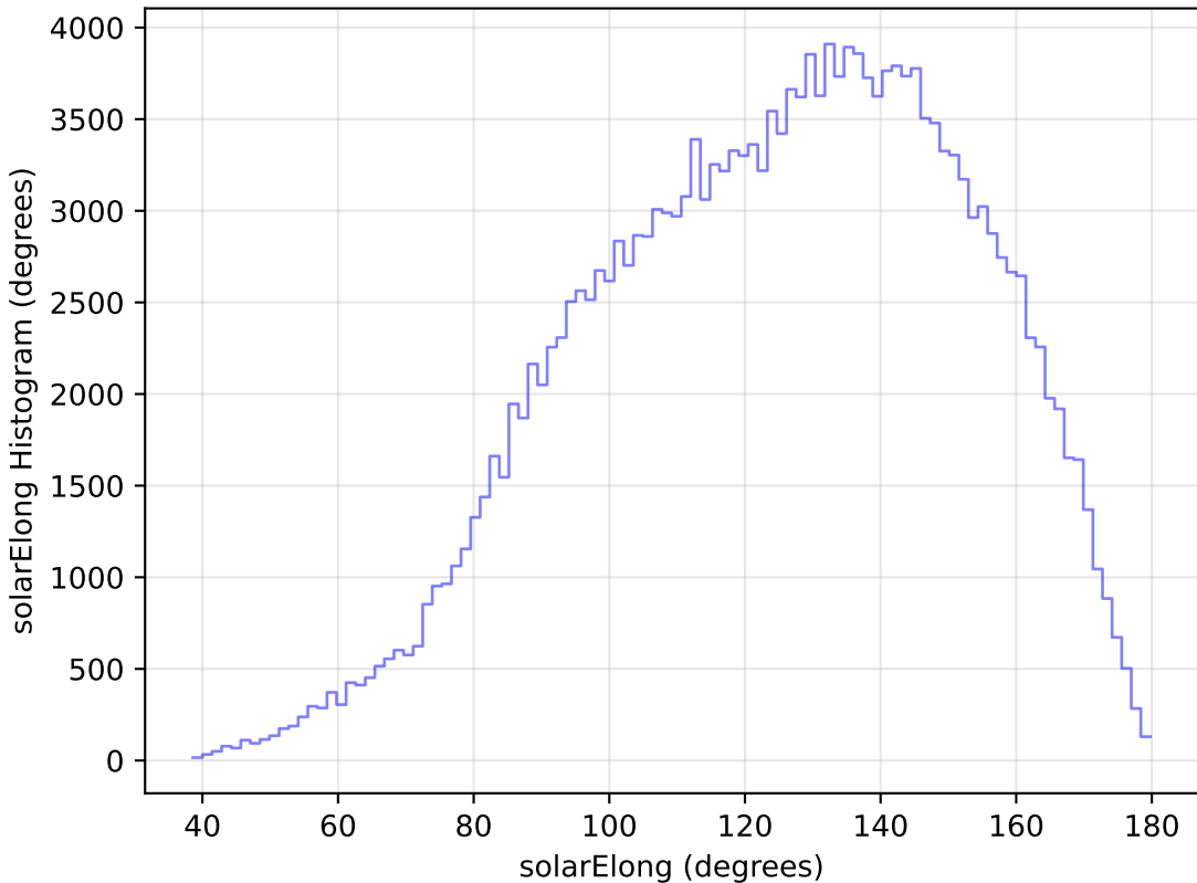
too_elab_r64_d3_ugrizy_v3.4_10yrs All sky g band: solarElong Histogram
