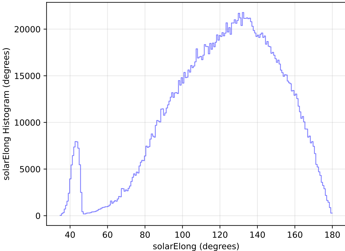
too_elab_r64_d3_ugrizy_v3.4_10yrs All sky all bands: solarElong Histogram
