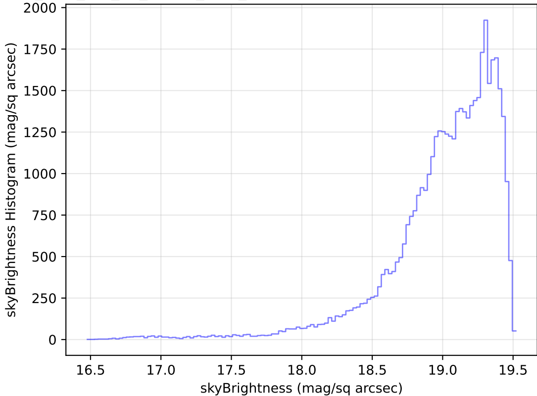
too_elab_r64_d3_ugrizy_v3.4_10yrs Yr 1 z band: skyBrightness Histogram
