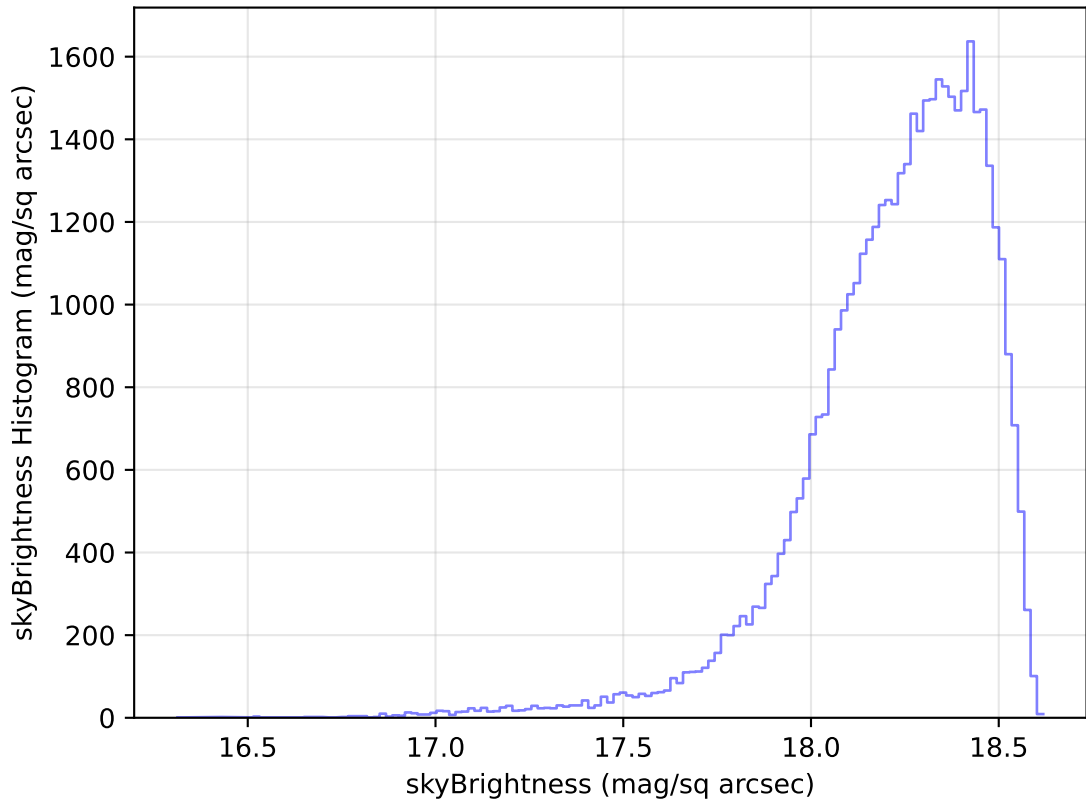
too_elab_r64_d3_ugrizy_v3.4_10yrs Yr 1 y band: skyBrightness Histogram
