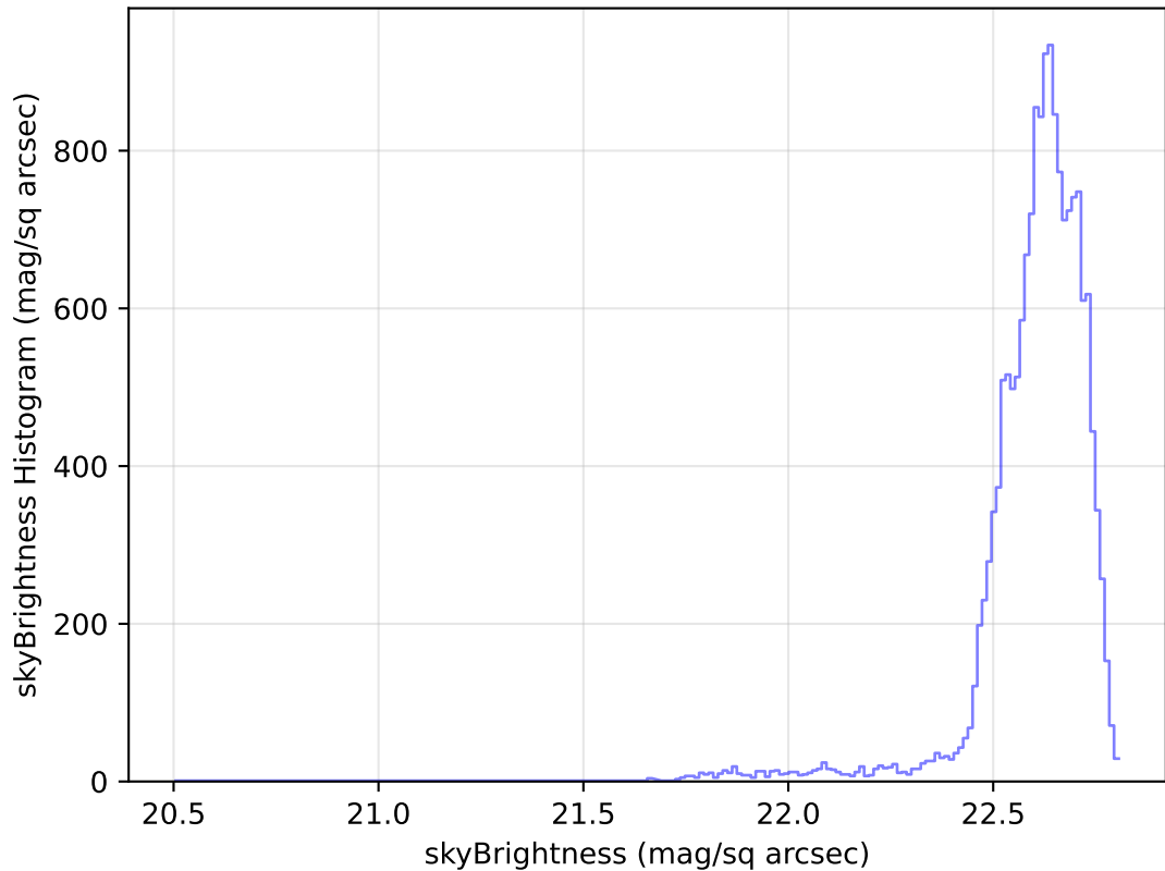
too_elab_r64_d3_ugrizy_v3.4_10yrs Yr 1 u band: skyBrightness Histogram
