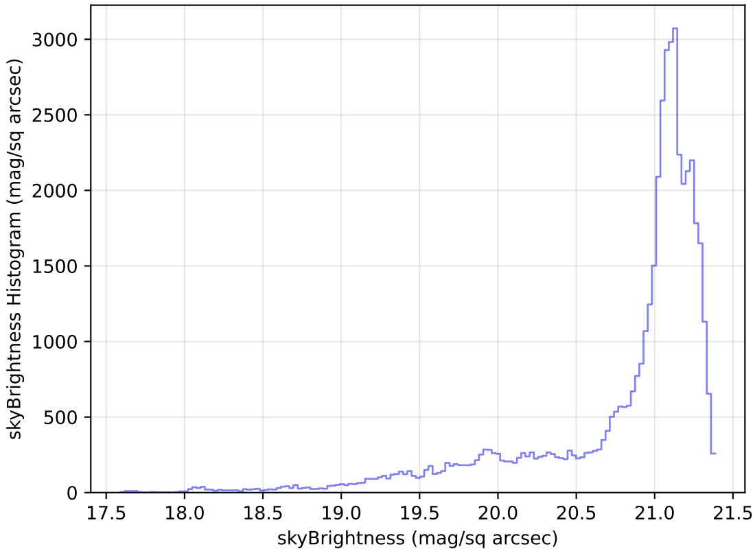
too_elab_r64_d3_ugrizy_v3.4_10yrs Yr 1 r band: skyBrightness Histogram
