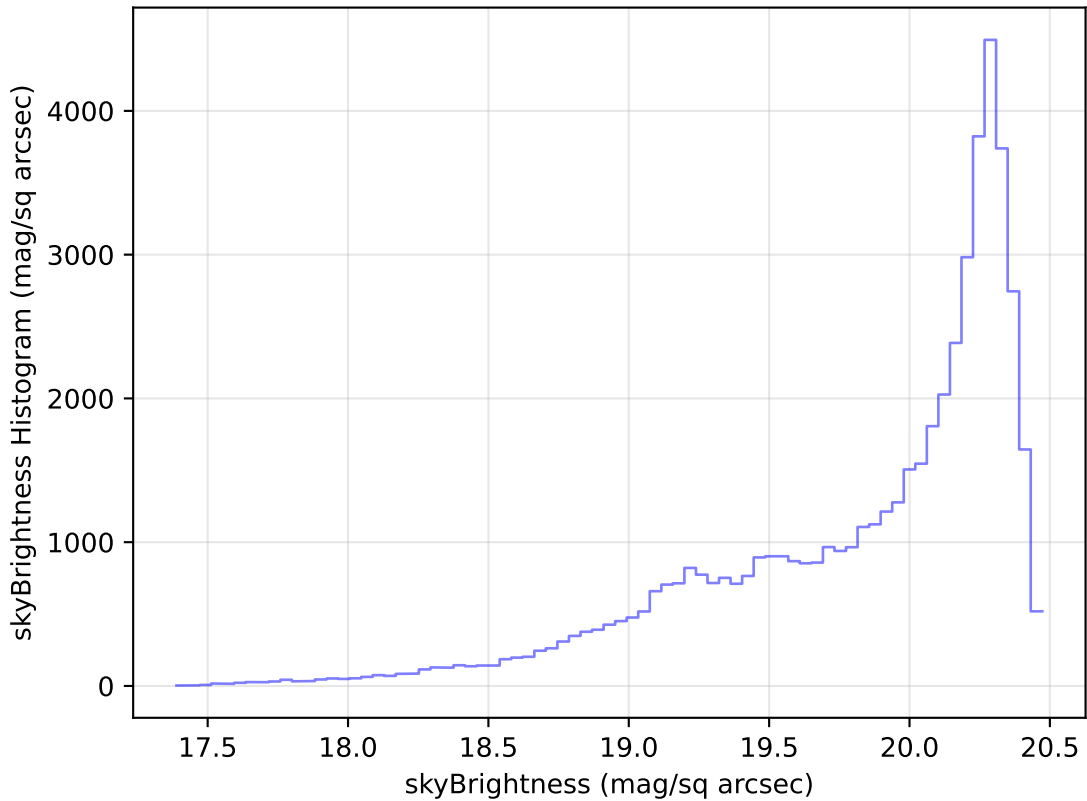
too_elab_r64_d3_ugrizy_v3.4_10yrs Yr 1 i band: skyBrightness Histogram
