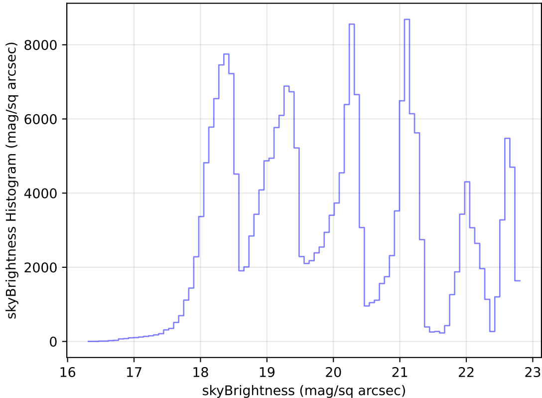
too_elab_r64_d3_ugrizy_v3.4_10yrs Yr 1 all bands: skyBrightness Histogram
