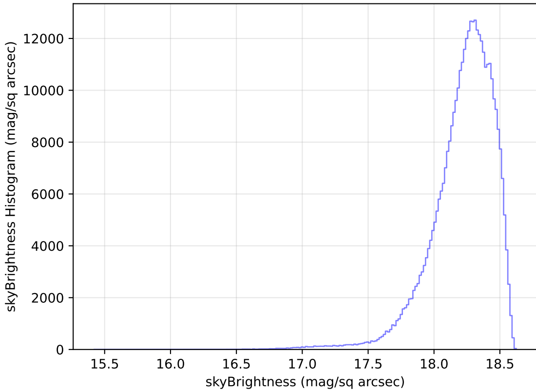
too_elab_r64_d3_ugrizy_v3.4_10yrs WFD y band: skyBrightness Histogram
