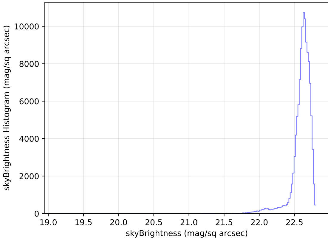
too_elab_r64_d3_ugrizy_v3.4_10yrs WFD u band: skyBrightness Histogram
