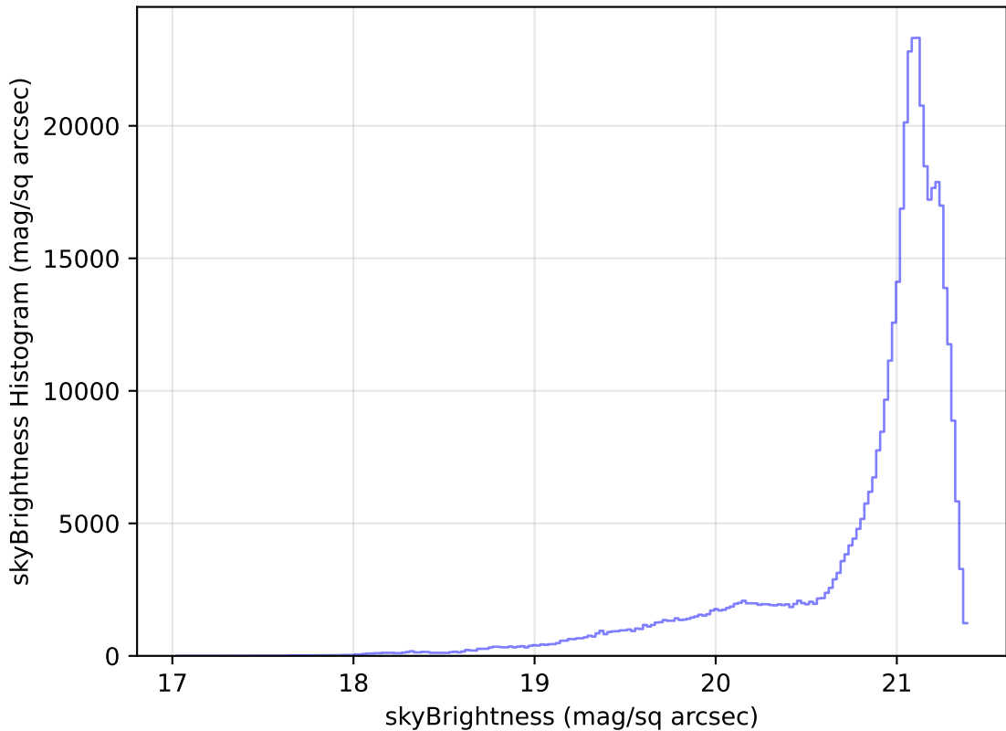
too_elab_r64_d3_ugrizy_v3.4_10yrs WFD r band: skyBrightness Histogram
