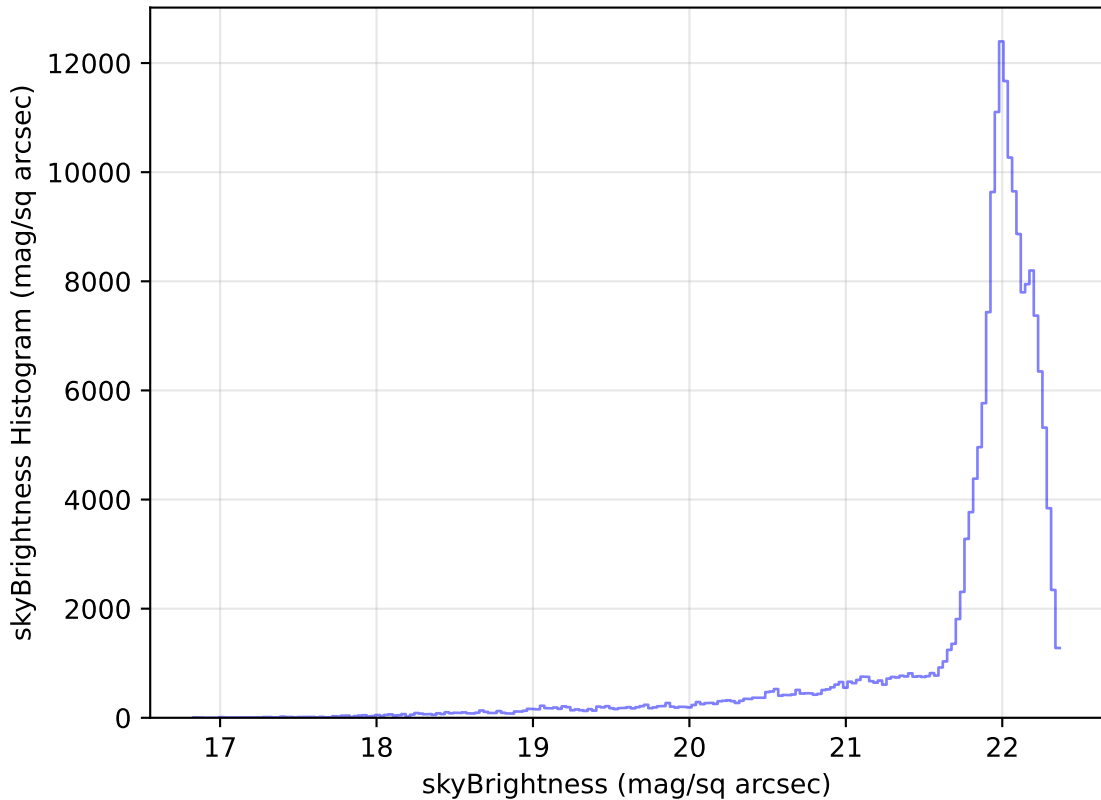
too_elab_r64_d3_ugrizy_v3.4_10yrs WFD g band: skyBrightness Histogram
