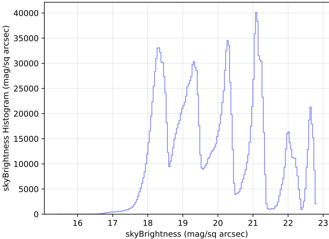
too_elab_r64_d3_ugrizy_v3.4_10yrs WFD all bands: skyBrightness Histogram
