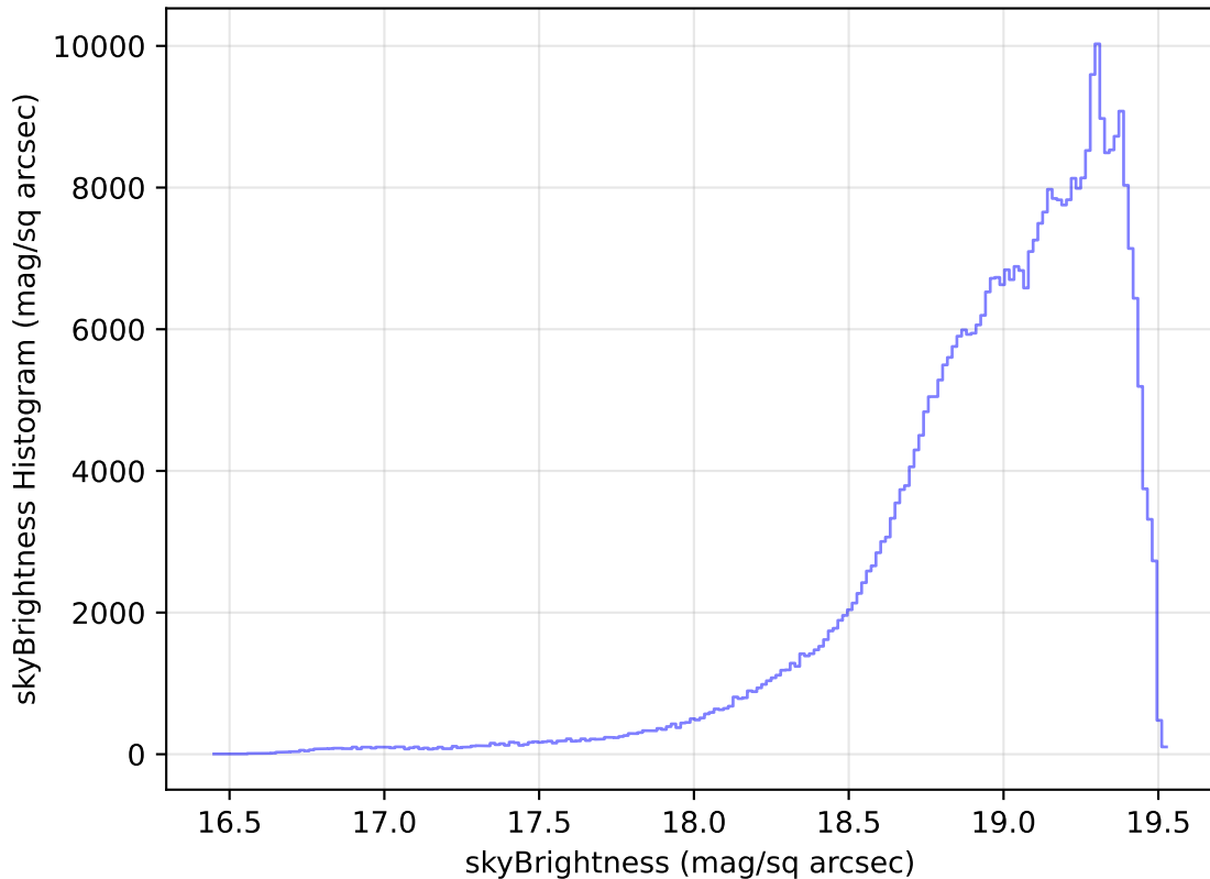
too_elab_r64_d3_ugrizy_v3.4_10yrs All sky z band: skyBrightness Histogram
