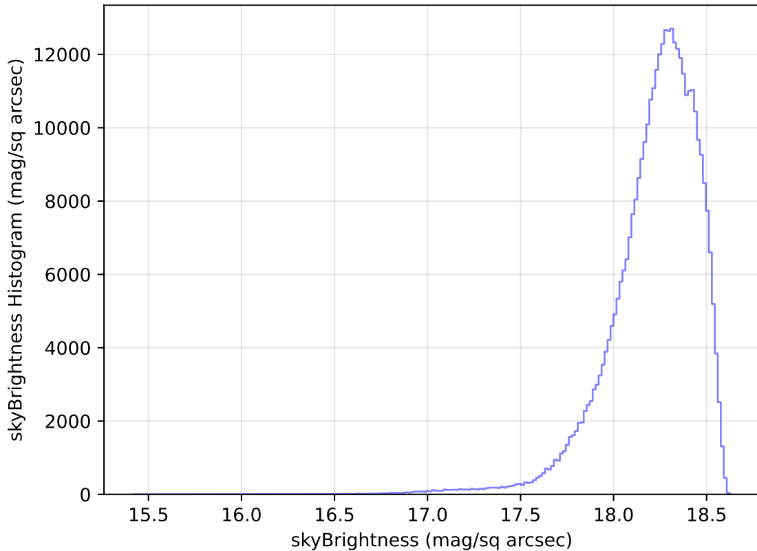
too_elab_r64_d3_ugrizy_v3.4_10yrs All sky y band: skyBrightness Histogram
