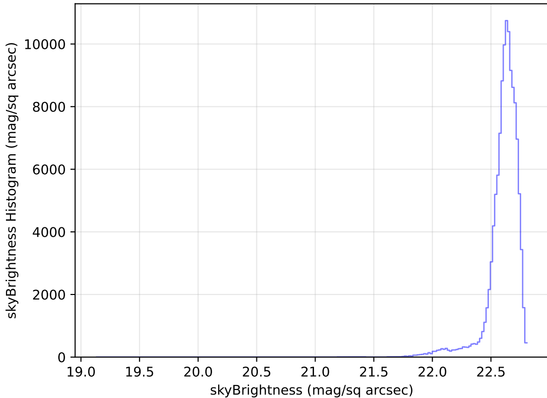
too_elab_r64_d3_ugrizy_v3.4_10yrs All sky u band: skyBrightness Histogram
