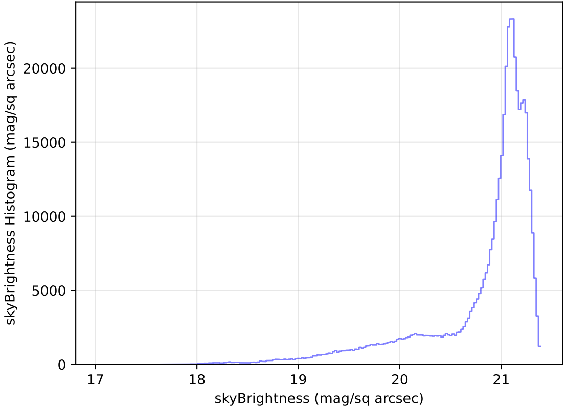
too_elab_r64_d3_ugrizy_v3.4_10yrs All sky r band: skyBrightness Histogram
