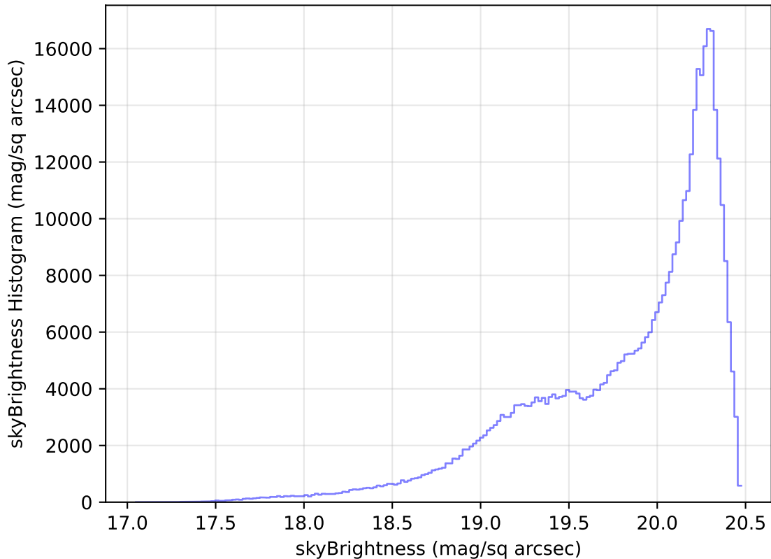
too_elab_r64_d3_ugrizy_v3.4_10yrs All sky i band: skyBrightness Histogram
