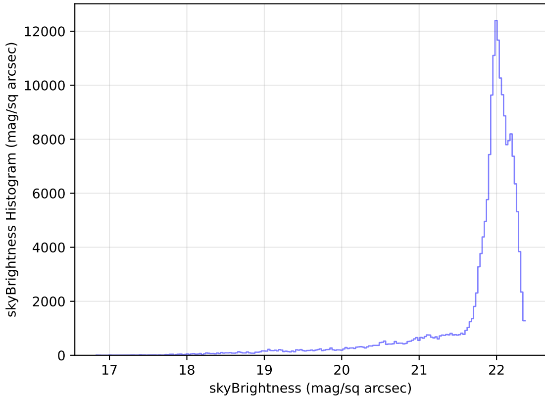
too_elab_r64_d3_ugrizy_v3.4_10yrs All sky g band: skyBrightness Histogram
