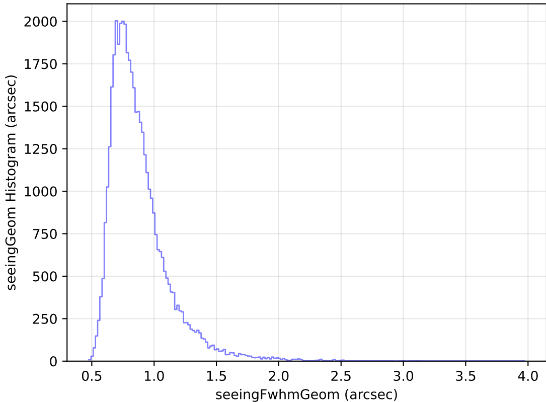
too_elab_r64_d3_ugrizy_v3.4_10yrs Yr 1 z band: seeingGeom Histogram
