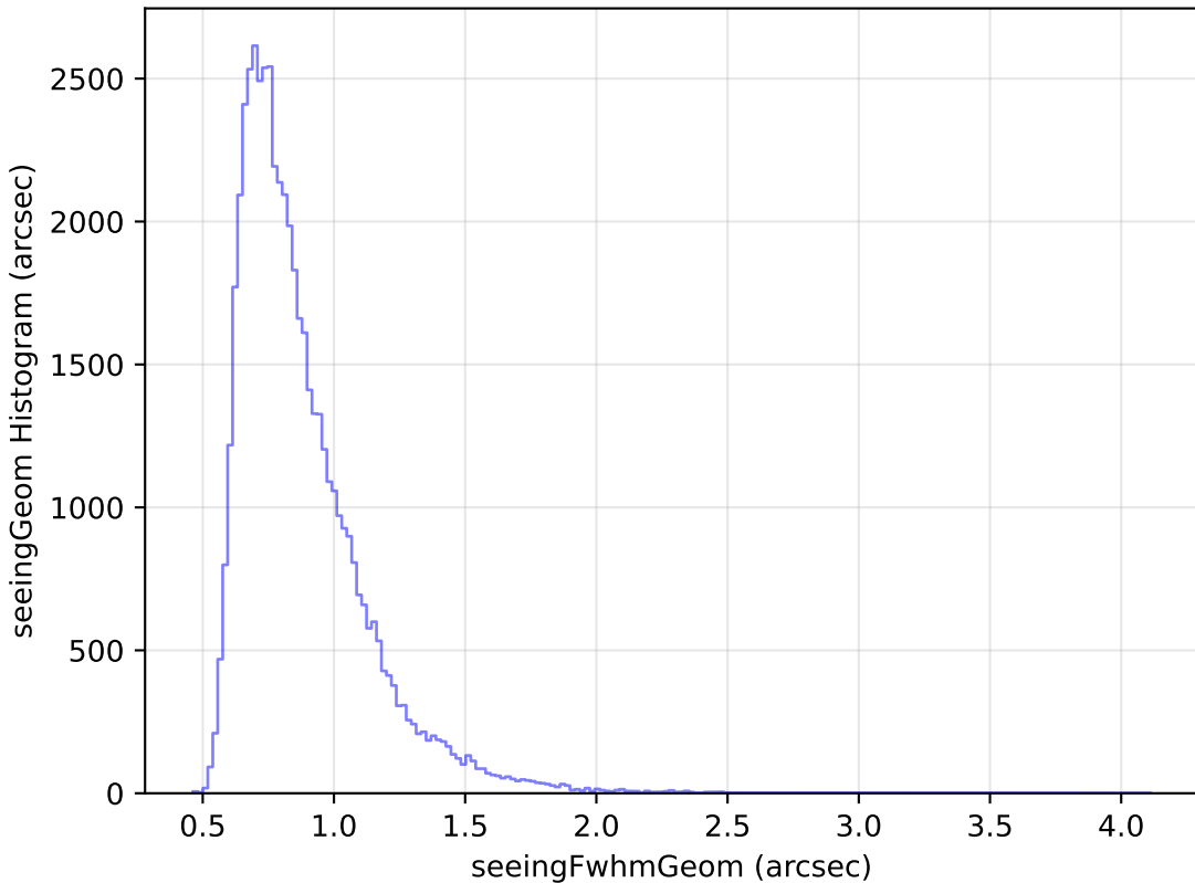
too_elab_r64_d3_ugrizy_v3.4_10yrs Yr 1 i band: seeingGeom Histogram
